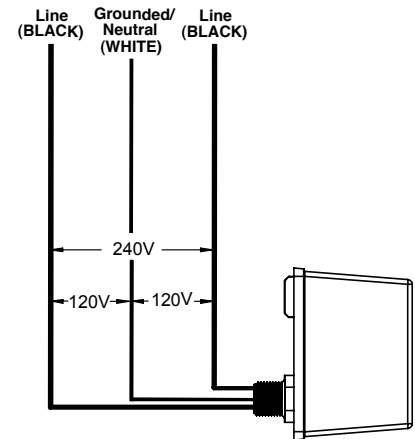
120/240 VAC Three wire with grounded neutral.
